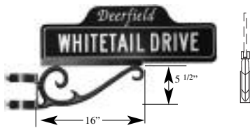
item# TSCR for use with 3" O/D round poles Scroll: 16" long, 5 1/2" high
