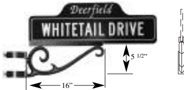
item# TSCR-600 for use with 4" O/D round poles Scroll: 16" long 5 1/2" high
